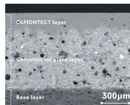
CEFIONTECT toilet micrograph *1µm=0.001mm
