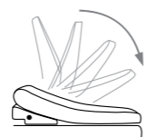
Soft closing
