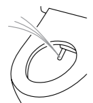
Rear cleansing
